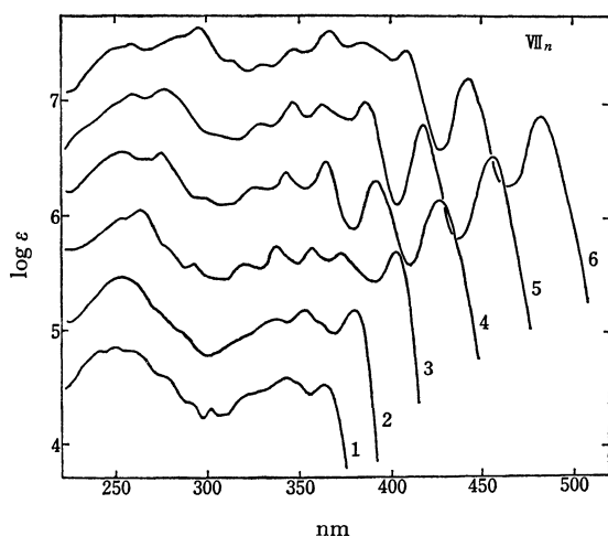
Fig. 4. Absorption curves of 9,9'-diphenanthrylpoly-ynes ( VII_1 — VII_6 ). Each curve, except for the lowest one, has been displaced upward by a 0.5 log \epsilon unit increment from one immediately below it.
